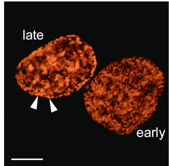
Figure 1 Timing of replication correlates with chromatin location. HeLa cells were briefly pulsed with Cy3-dUTP to mark actively replicating regions of chromatin, then fixed and imaged on a fluorescence microscope. The cell on the left is late in S-phase and preferentially replicating heterochromatic regions, with those in the nuclear periphery marked by arrowheads. The cell on the right is at an earlier stage of S phase, when predominantly internal chromatin is replicated. See [15] and references therein for further details. Scale bar = 5 \mu m.
